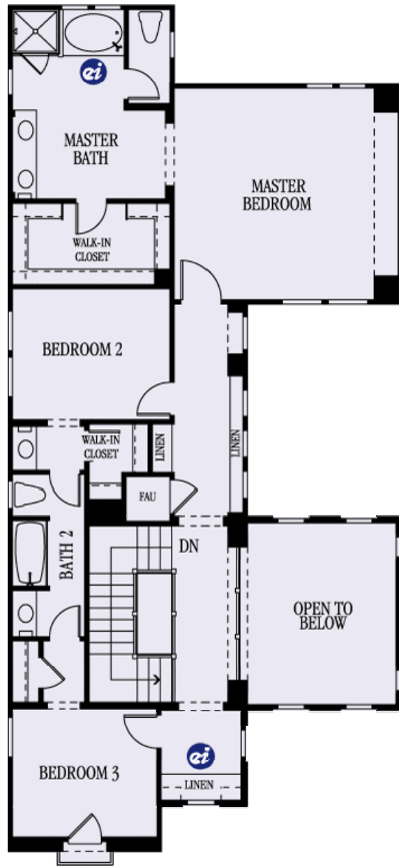
SECOND FLOOR
